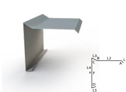
Attikakappe 1
