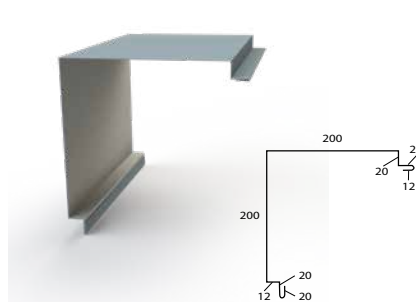
Attikakappe 2
