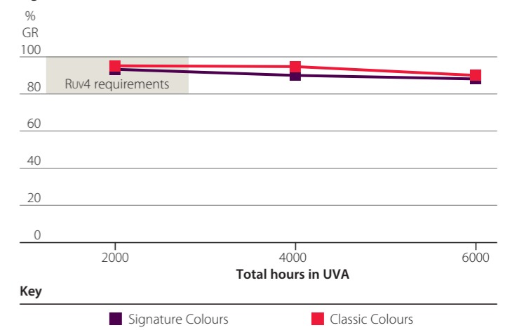
Figure 27. % Gloss Retention for Colorcoat HPS200 Ultra® in UVA
