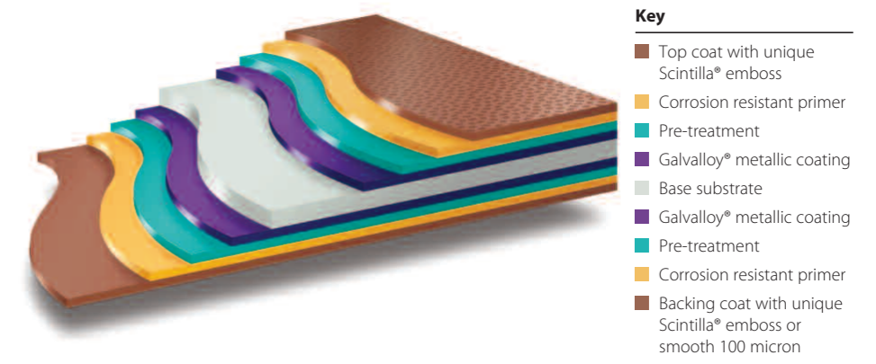
Figure 5. Double sided Colorcoat HPS200 Ultra® by Tata Steel
