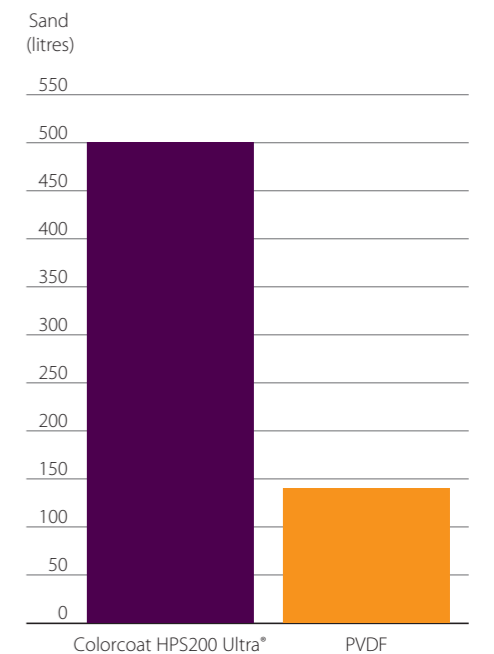
Figure 11. Abrasion resistance comparison (ASTM D968:2001)
